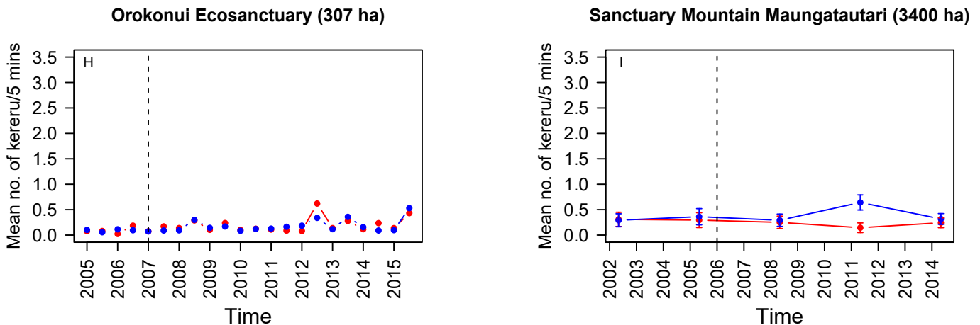
Figure 2. Long-term responses of kererū in ring-fenced ecosanctuaries. The blue points are kererū counts from the sanctuary site, and the red points are kererū counts from a nearby non-treatment site. Vertical dotted lines show when eradication occurred. Error bars are 95% confidence intervals.
