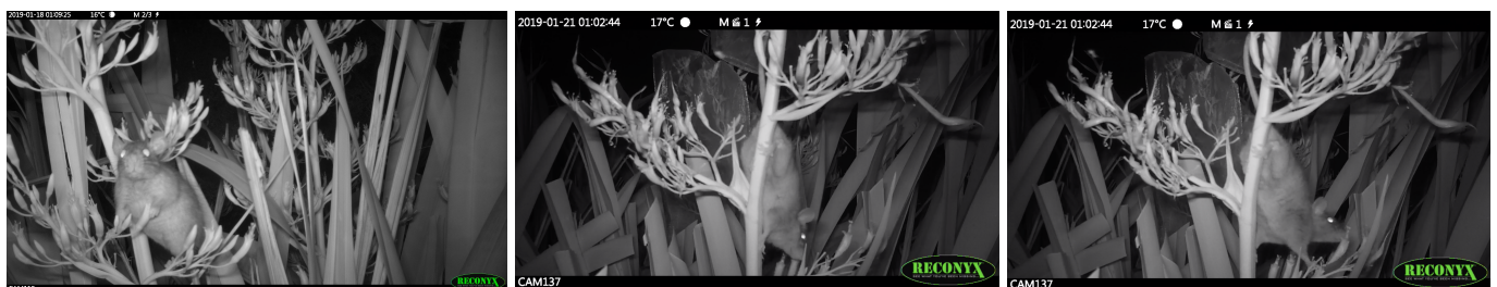
Figure 1. Photos from across multiple nights and camera traps, show a ship rat climbing across and appearing to feed from a mountain flax flower and reaching across to another open flower. During the feeding and when it reaches the other flower, the rat appears to contact the stamens and pistil, which extend above the petals and sepals.
